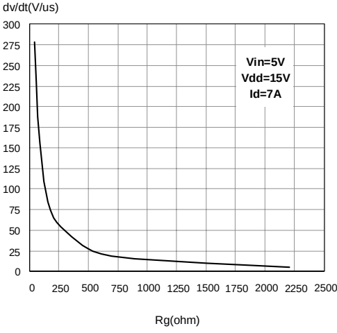
Figure 45. Turn off drain source voltage slope
