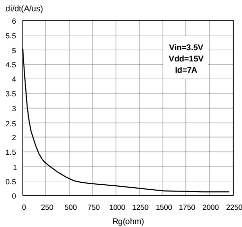
Figure 30. Turn On Current Slope
