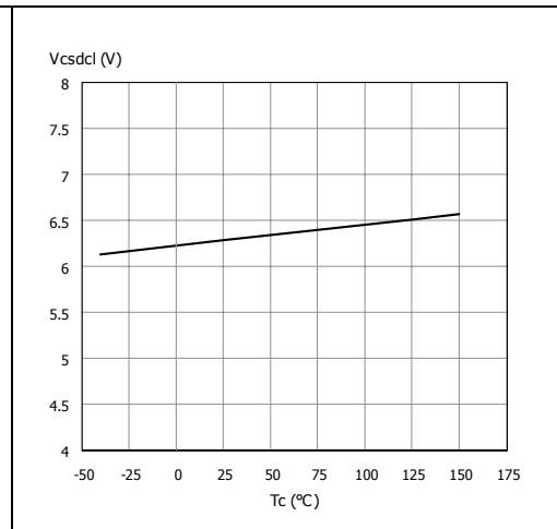
Figure 20. CS_DIS clamp voltage
