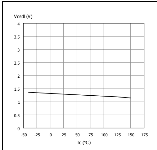
Figure 21. CS_DIS low level voltage
