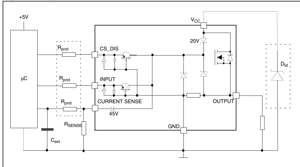
Figure 22. Application schematic
