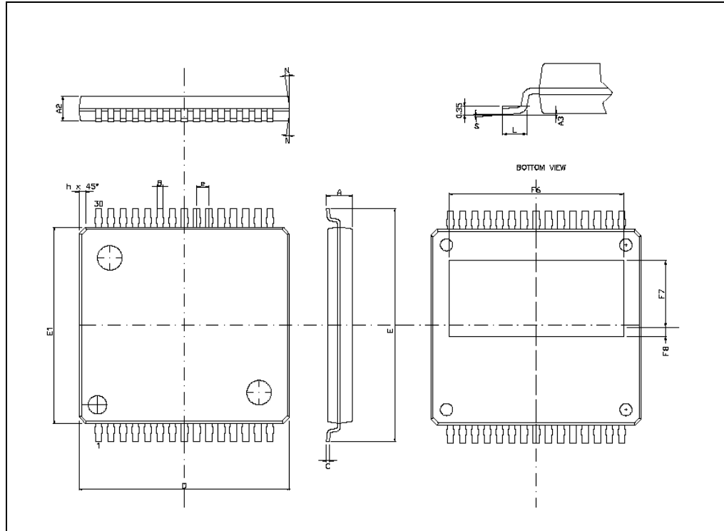
Figure 32. MultiPowerSO-30 outline
