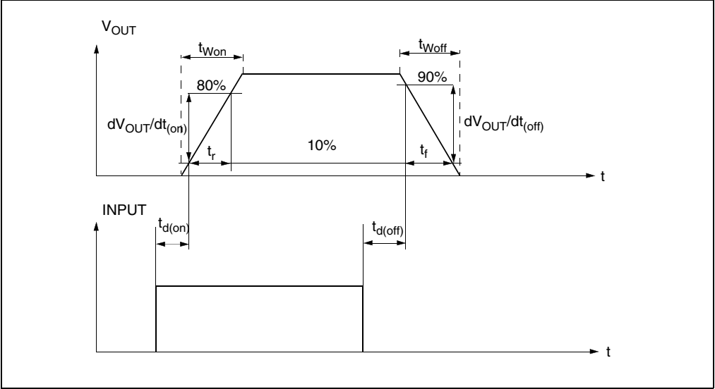
Figure 5. Switching characteristics
