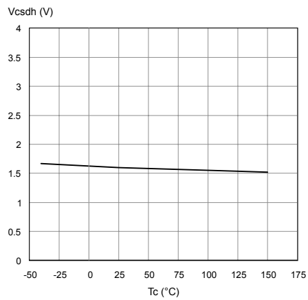
Figure 23. CS_DIS Clamp Voltage
