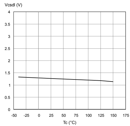
Figure 22. CS_DIS Low Level Voltage
