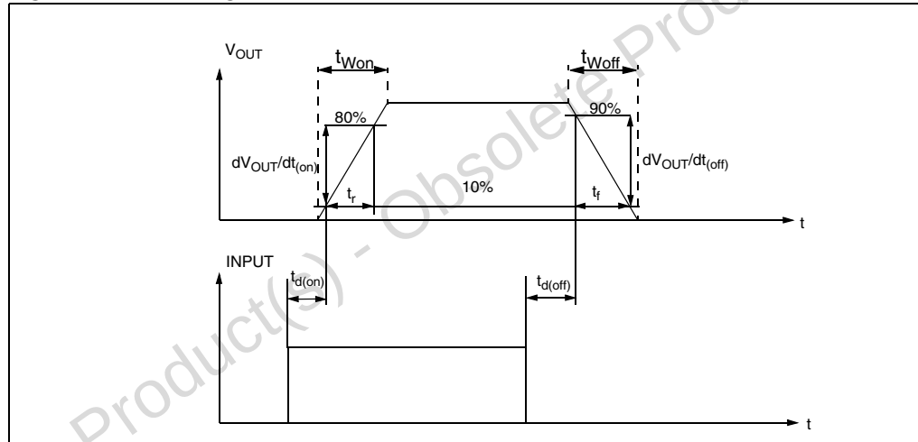
Figure 6. Switching characteristics
