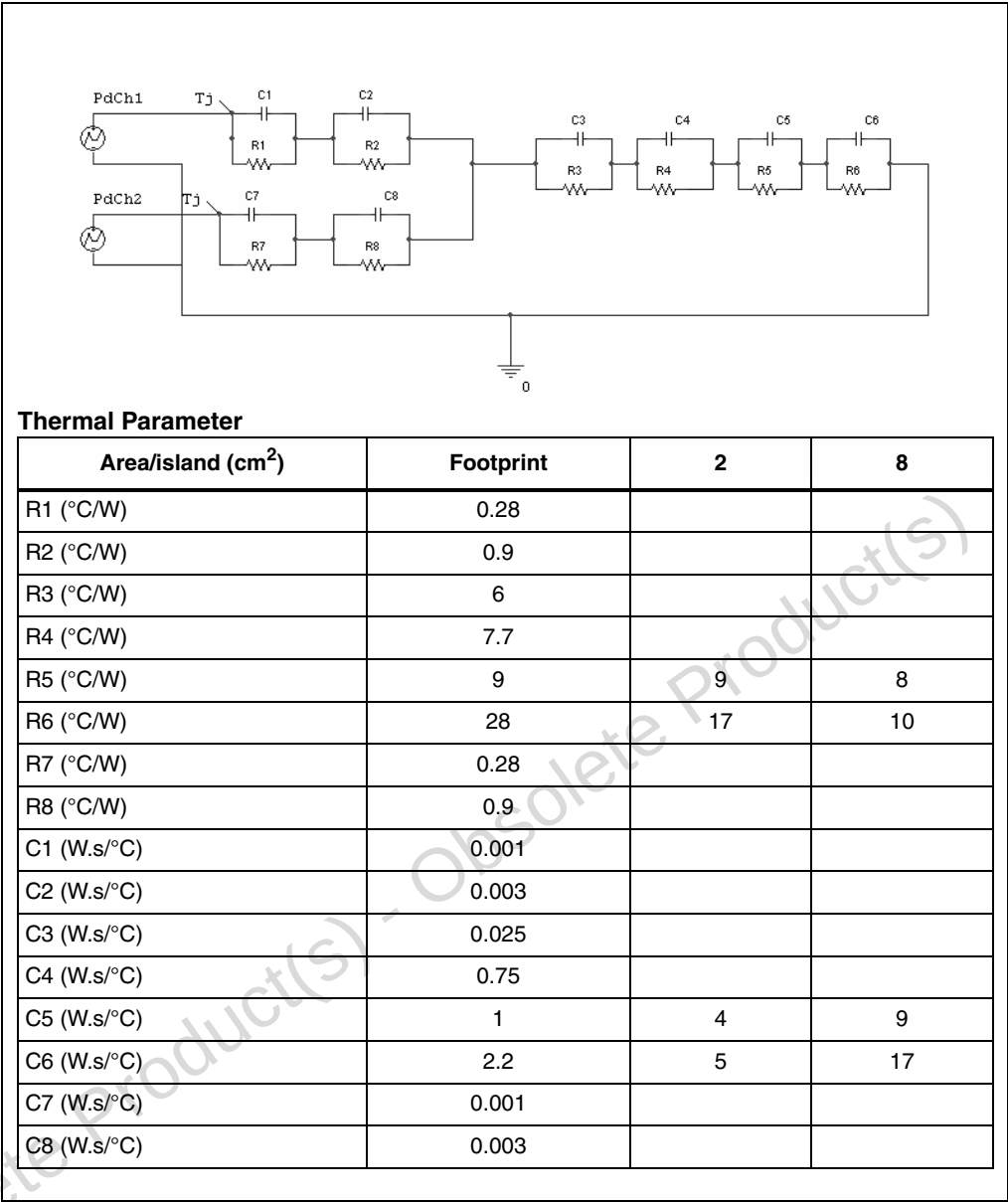
Figure 28. Thermal Fitting Model of a Single Channel HSD in PowerSSO-12
