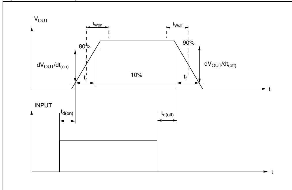
Figure 6. Switching characteristics
