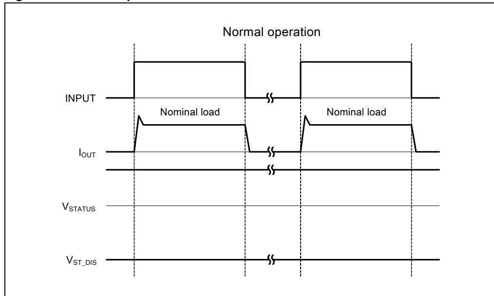
Figure 7. Normal operation
