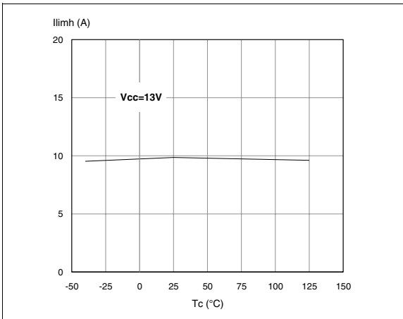
Figure 25. I_{LIM} vs T_{case}
