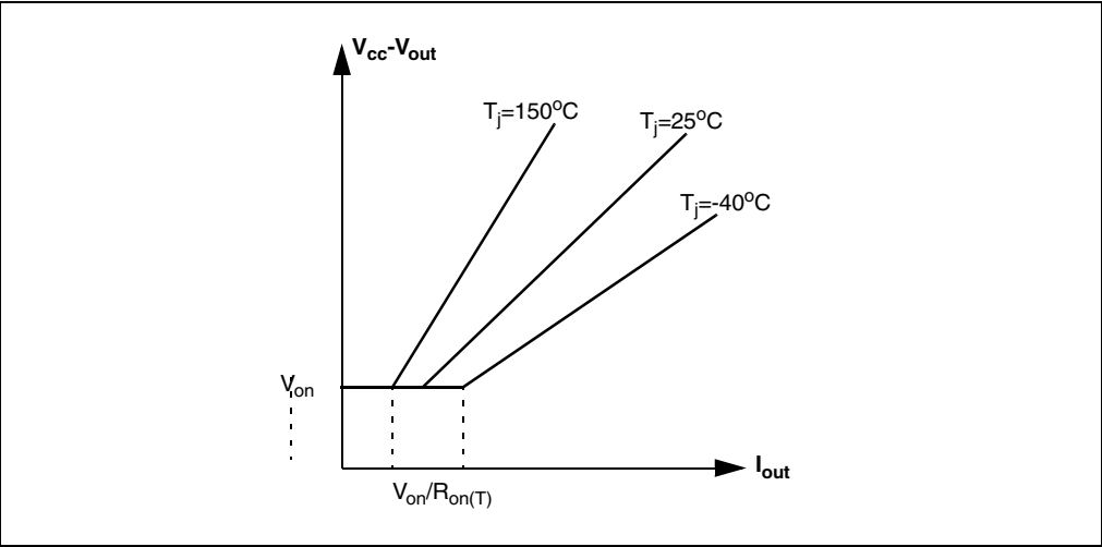
Figure 5. Output voltage drop limitation
