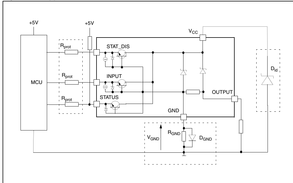
Figure 32. Application schematic
