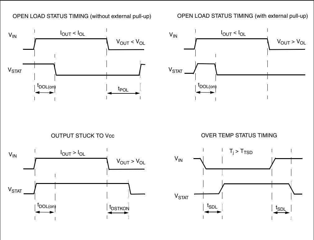
Figure 4. Status timings
