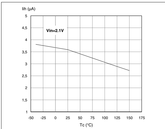
Figure 18. Input high level
