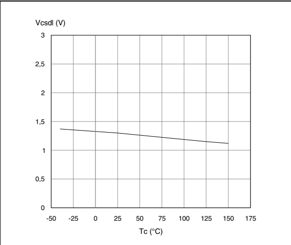
Figure 28. Low-level CS_DIS voltage
