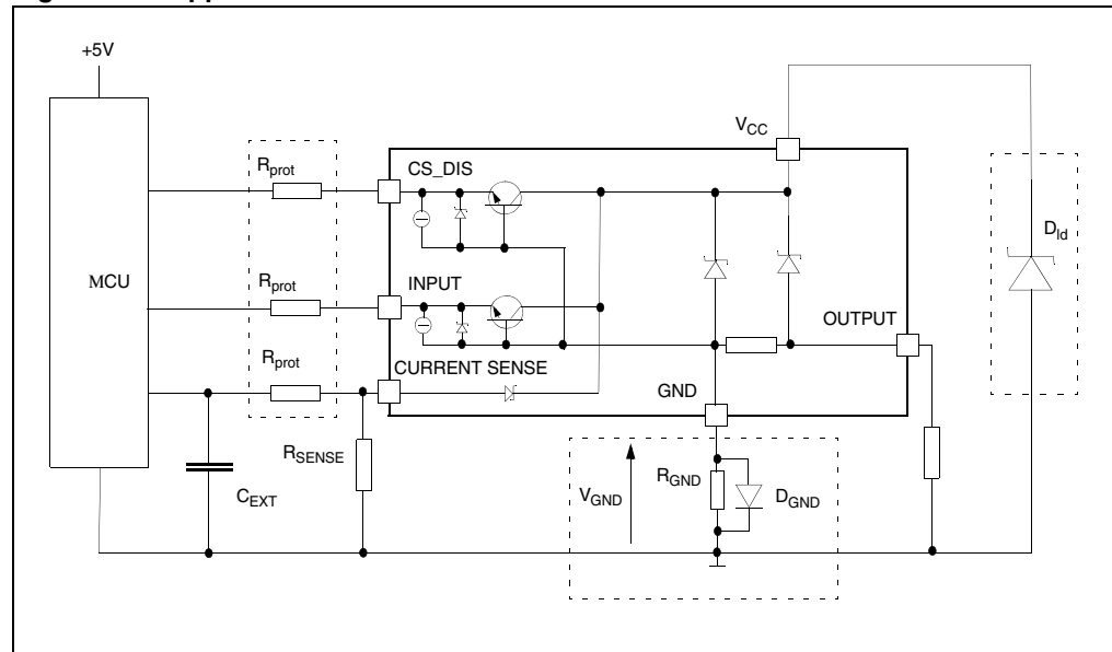
Figure 29. Application schematic (1)
