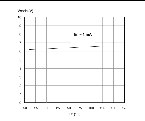
Figure 27. CS_DIS clamp voltage
