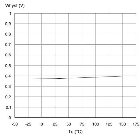
Figure 19. Hysteresis input voltage
