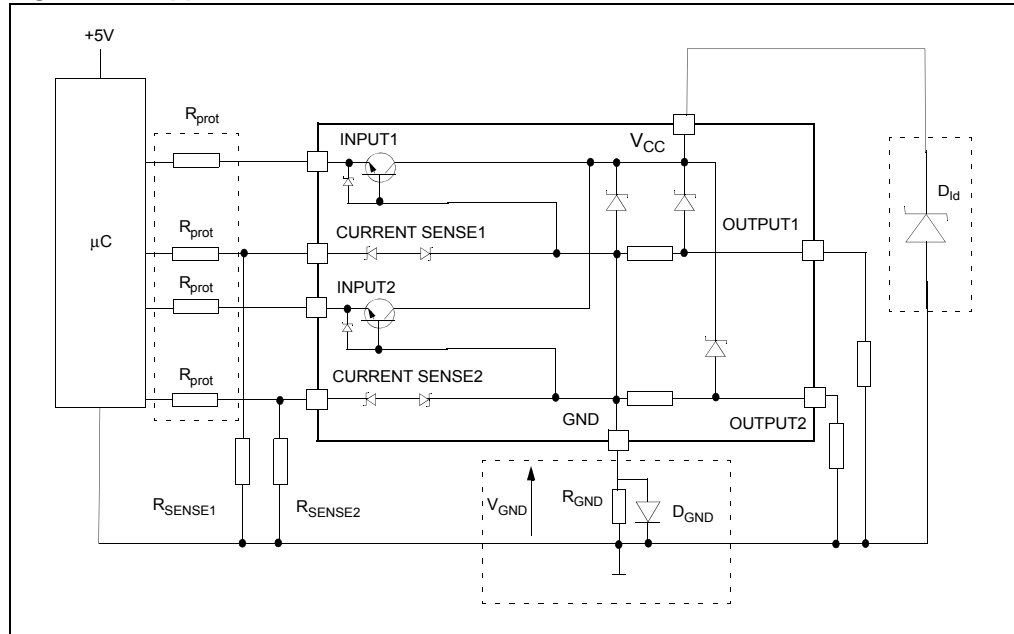
Figure 19. Application schematic
