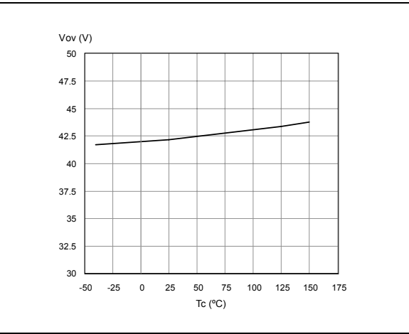
Figure 11. Overvoltage shutdown
