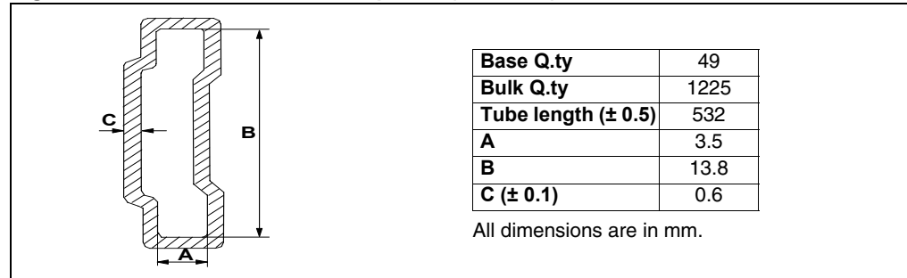
Figure 26. PowerSSO-24 tube shipment (no suffix)
