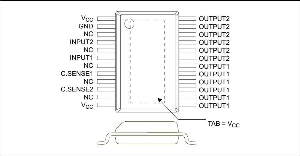
Figure 2. Configuration diagram (top view)
