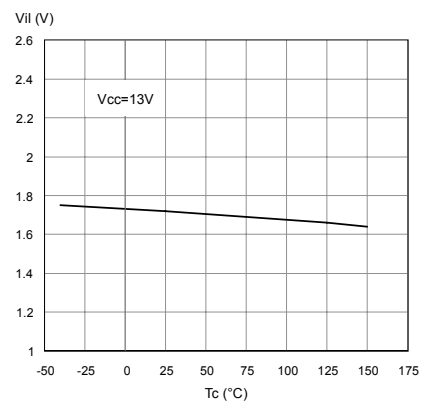
Figure 18. Input low level
