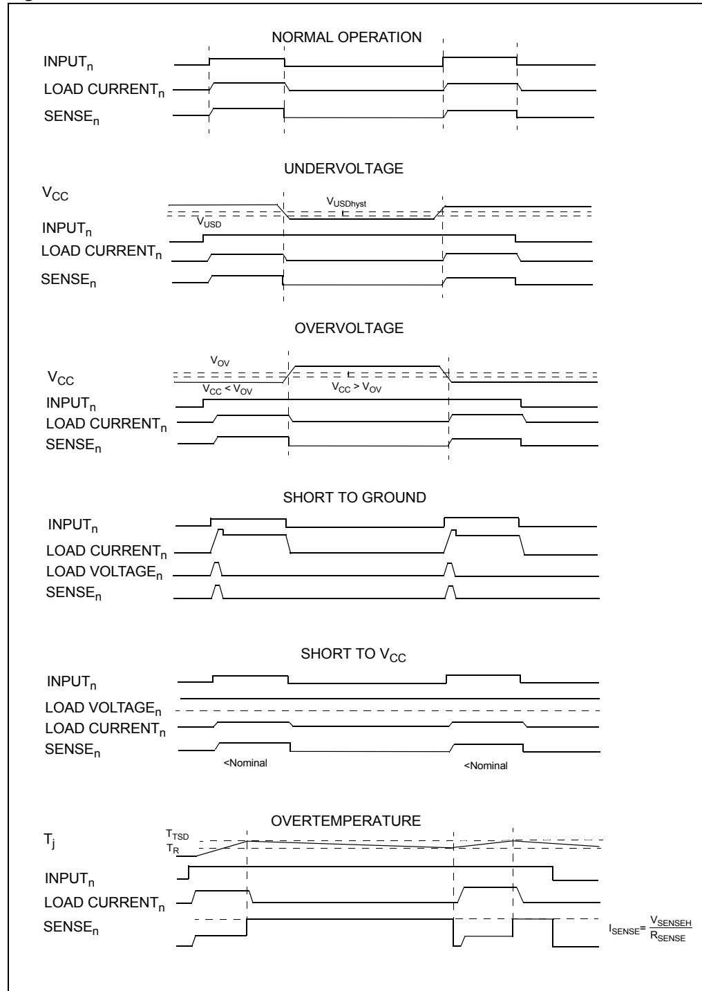
Figure 6. Waveforms
