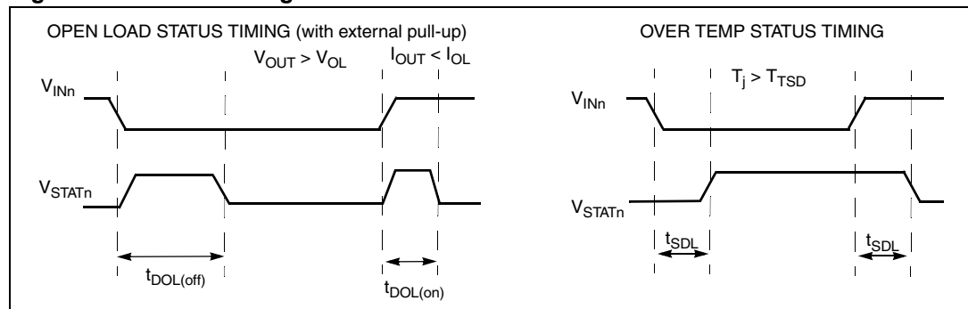
Figure 4. Status timings
