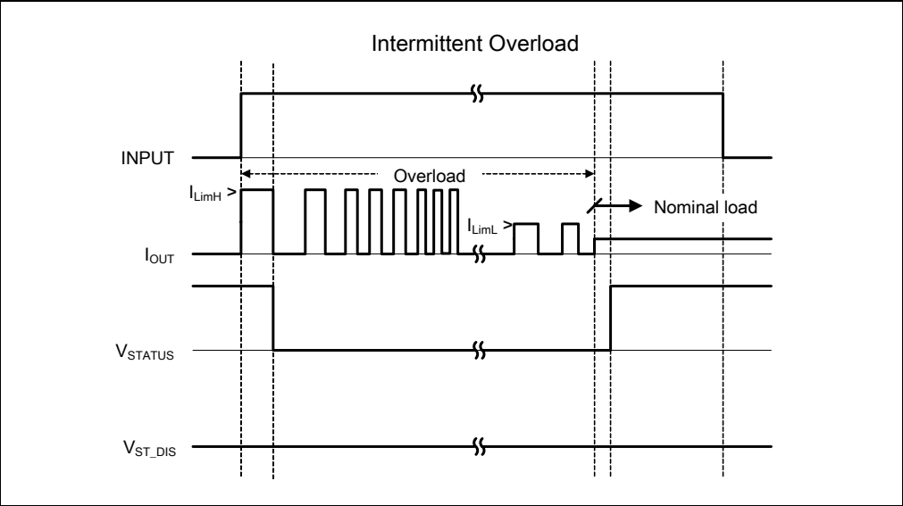
Figure 10. Intermittent overload
