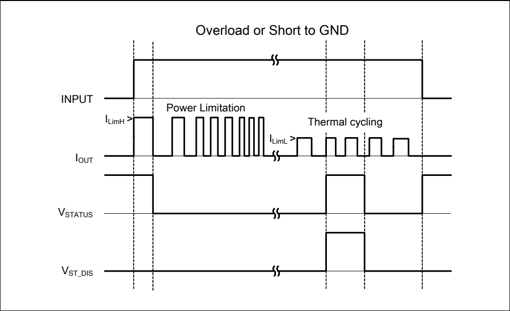
Figure 9. Overload or short to GND
