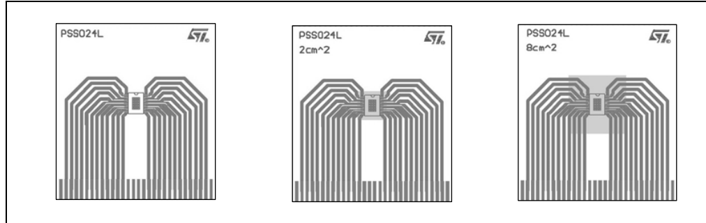
Figure 35. PowerSSO-24 PC board (1)
