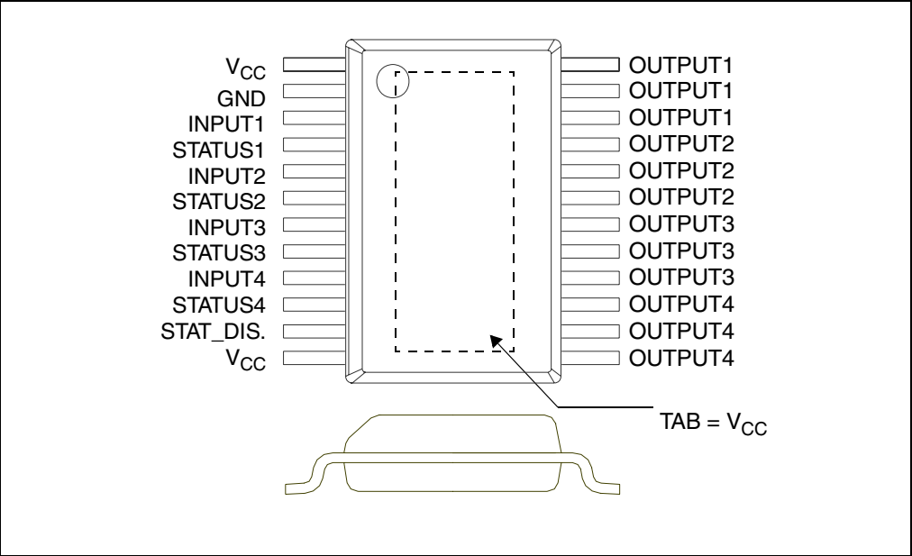
Figure 2. Configuration diagram (top view)
