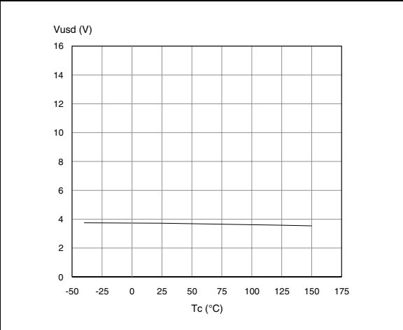
Figure 29. STAT_DIS clamp voltage
