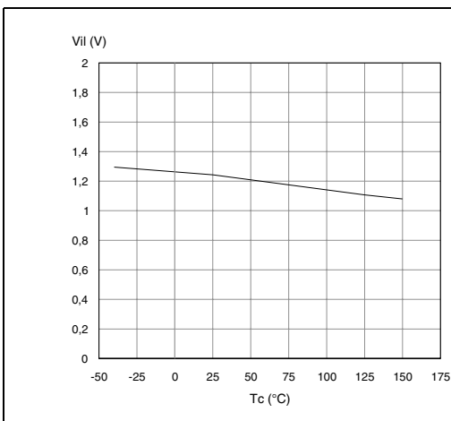
Figure 19. Input low level voltage
