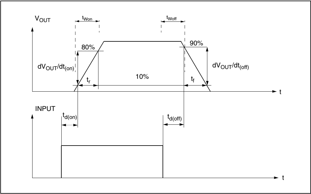
Figure 6. Switching characteristics
