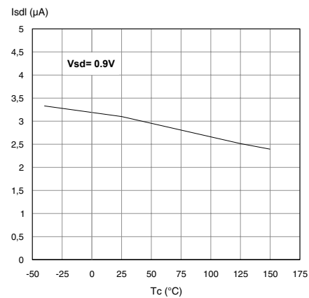
Figure 20. Low level STAT_DIS current
