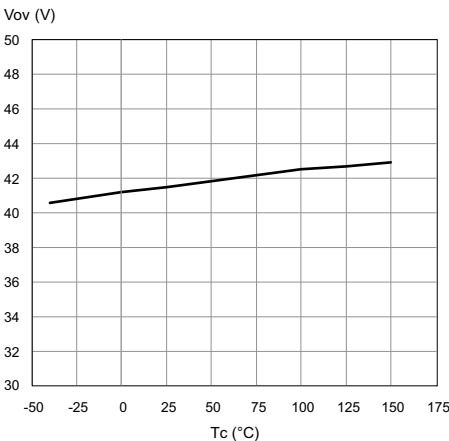
Figure 14. Overvoltage shutdown
