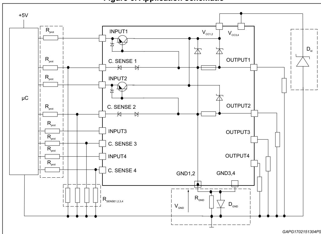
Figure 6. Application schematic
