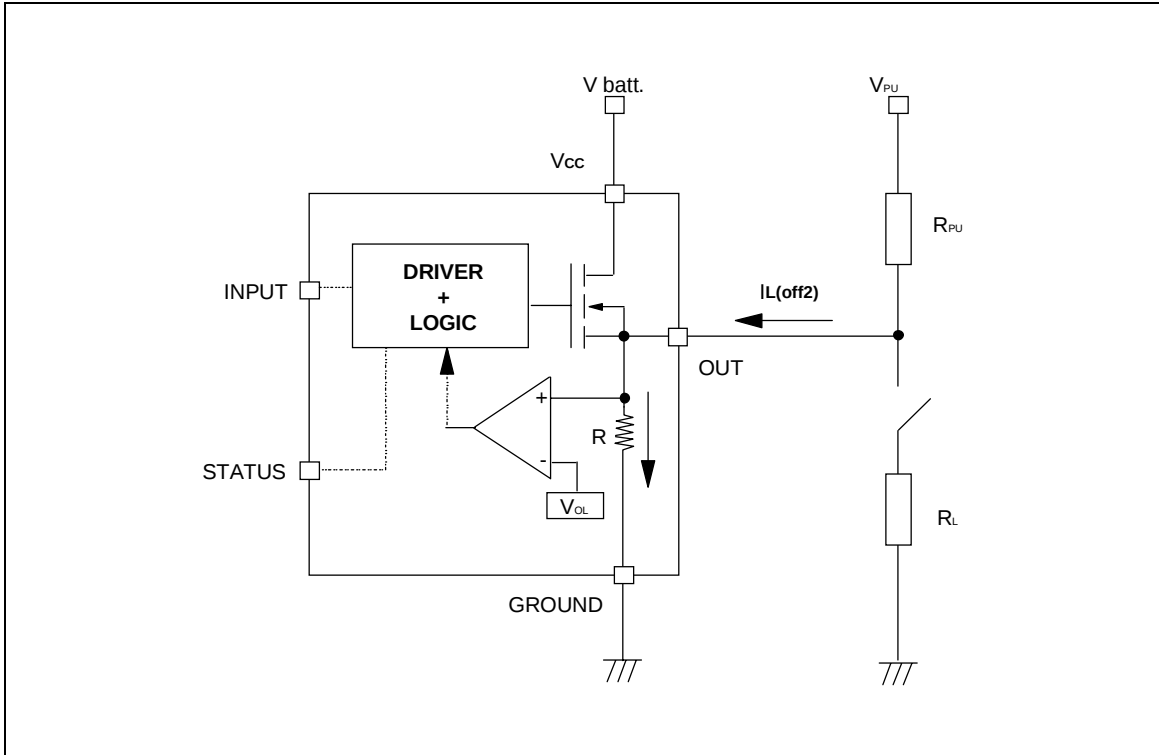
Figure 9. Open Load detection in off state
