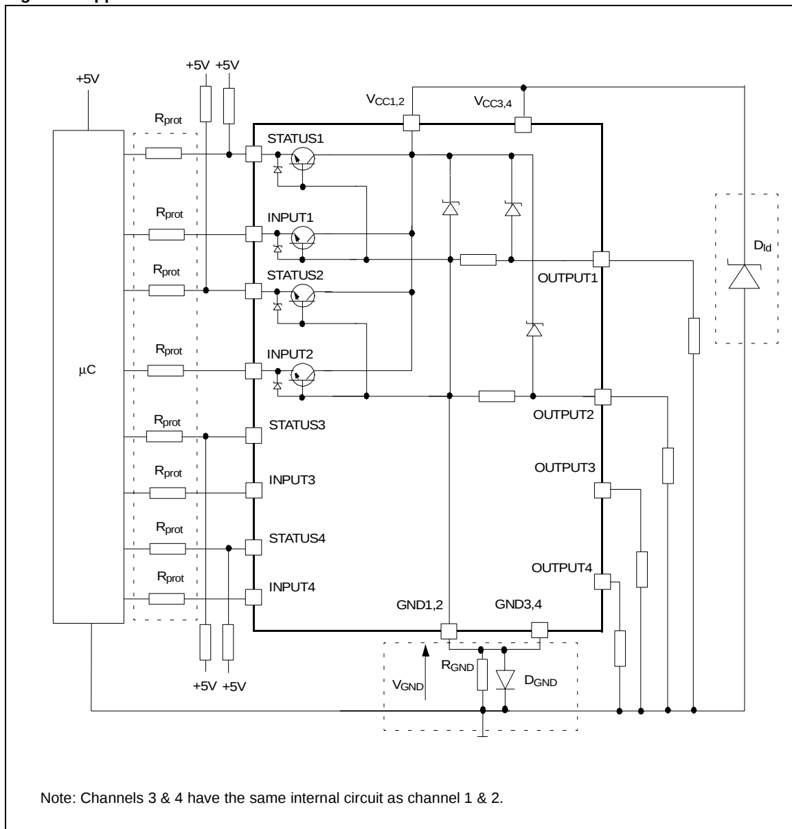
Figure 8. Application Schematic
