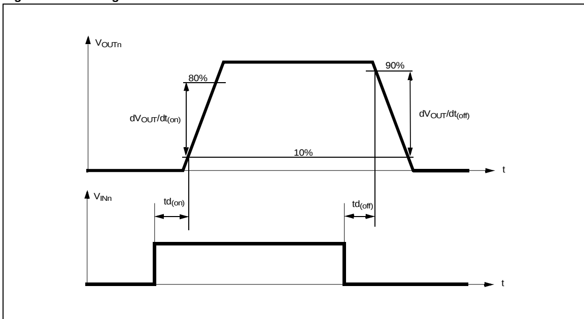
Figure 6. Switching time Waveforms
