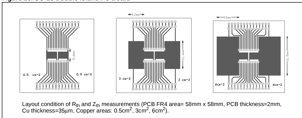
Figure 28. SO-28 Double Island PC Board
