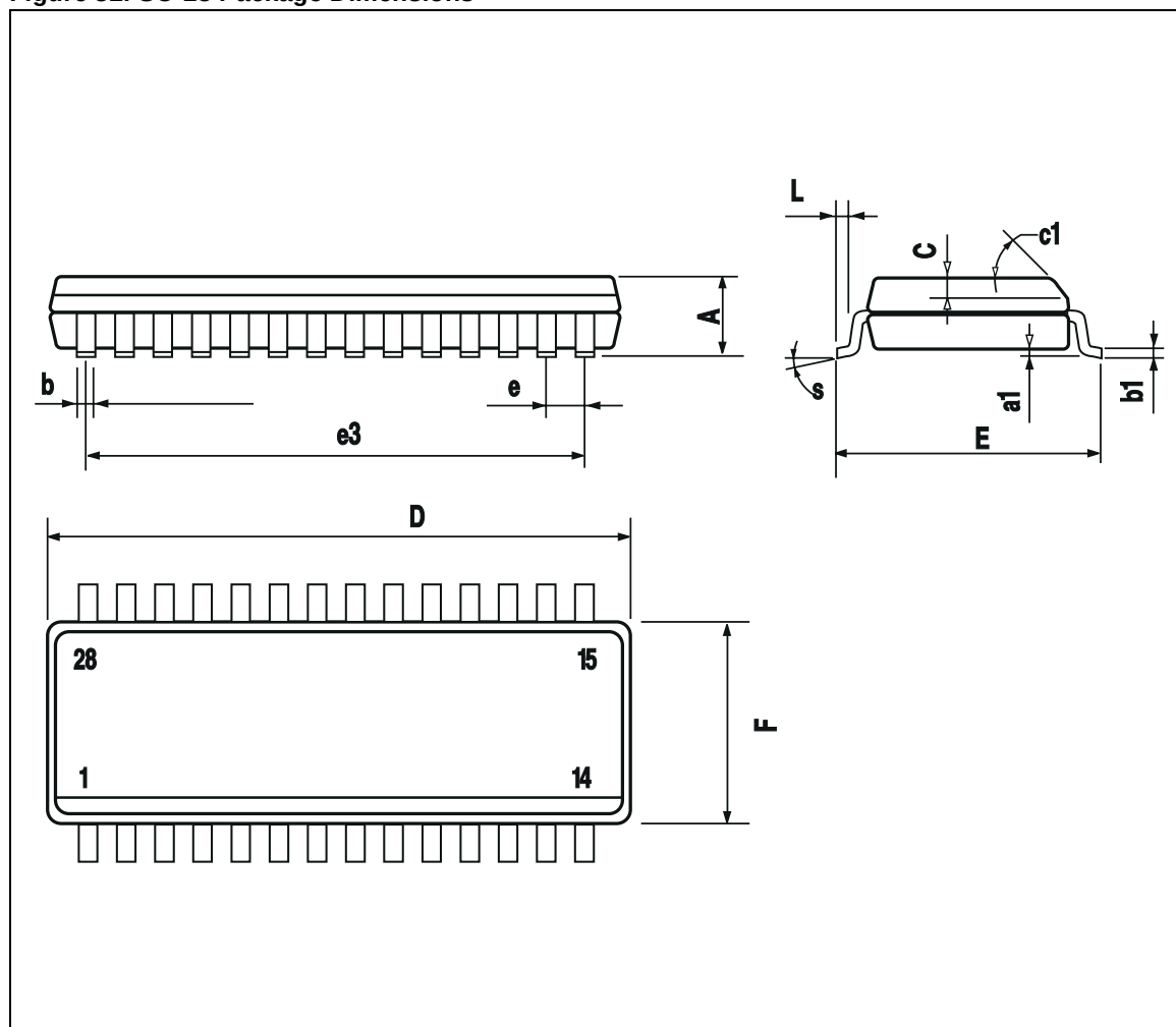
Figure 32. SO-28 Package Dimensions
