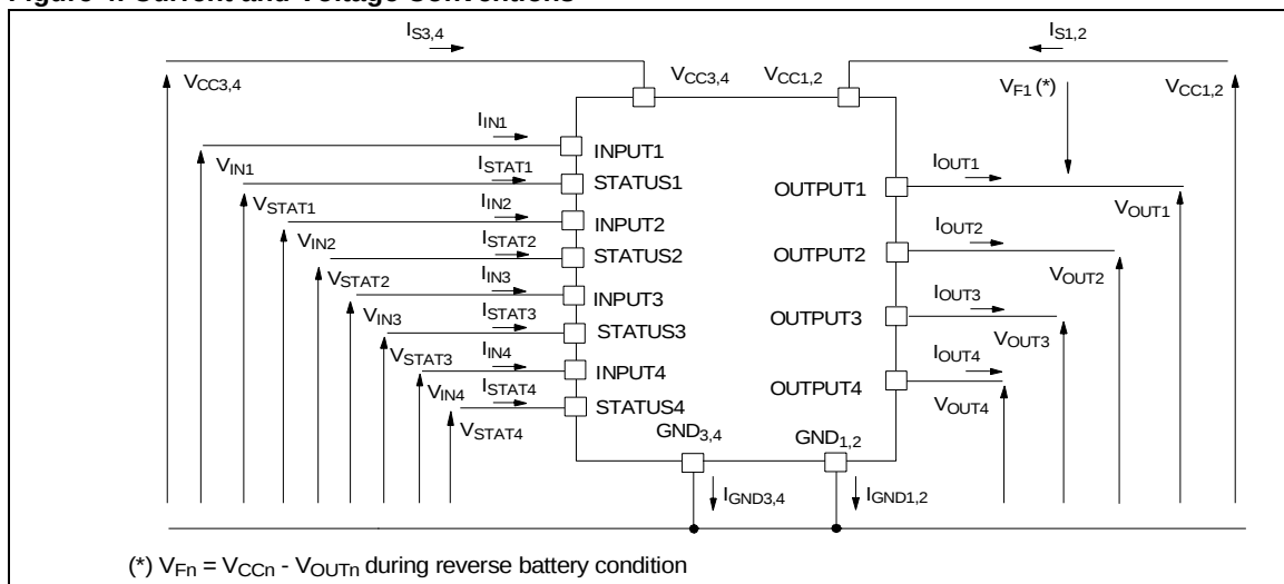
Figure 4. Current and Voltage Conventions
