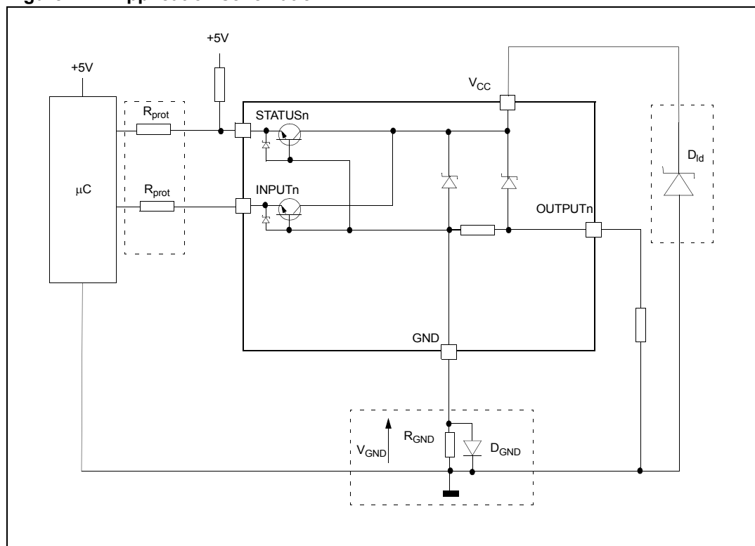
Figure 24. Application schematic
