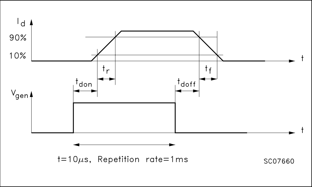
Figure 30. Waveforms
