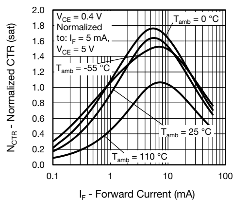
Fig. 13 - Current Transfer Ratio vs. Forward Current (non-saturated) Normalized to 1 mA at 25^\circ\text{C}
