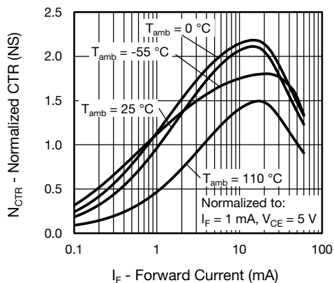
Fig. 12 - Current Transfer Ratio vs. Forward Current (saturated) Normalized to 1 mA at 25^\circ\text{C}
