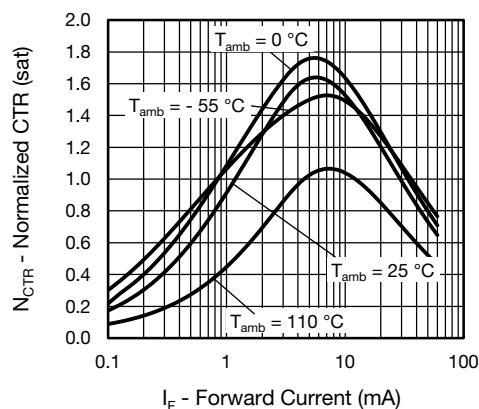
Fig. 11 - Current Transfer Ratio vs. Forward Current (saturated) normalized to 1 mA at 25 ^{\circ}C
