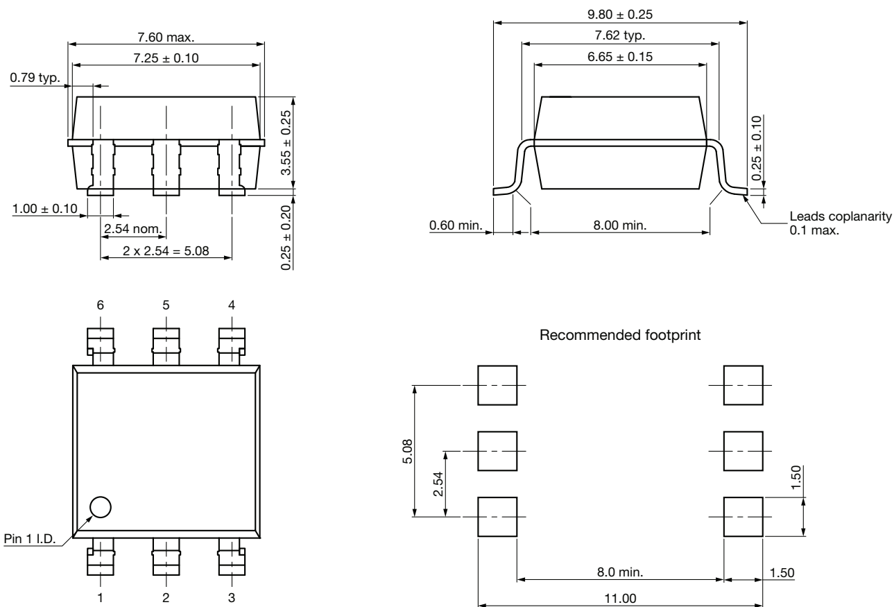
Fig. 16 - Package Drawings
