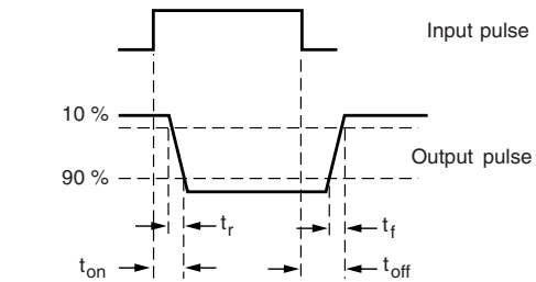
Fig. 4 - Test Circuit and Waveforms
