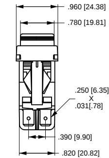
8 TERMINAL BASE W/BARRIERS
