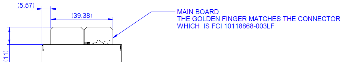
Figure 17- Mating Connector
