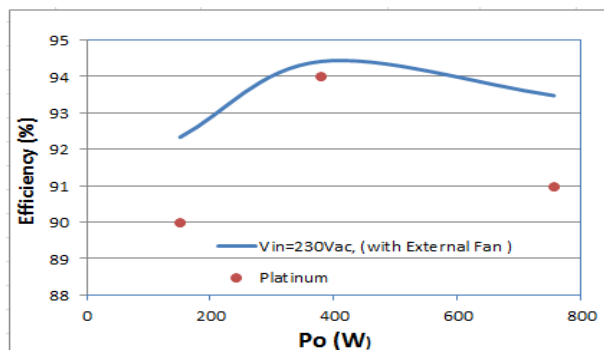
Figure 2 - Efficiency vs. Load current (ratio metric loading)
