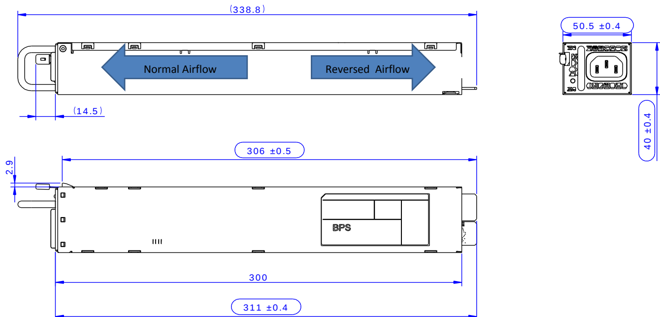
Figure 14 - Mechanical Drawing-Side/Top View
