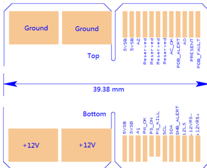
Figure 18 - Pin Assignment of DC Connector
