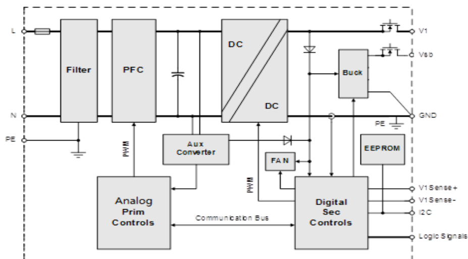
Figure 1 – PET750-12-050 Block Diagram
