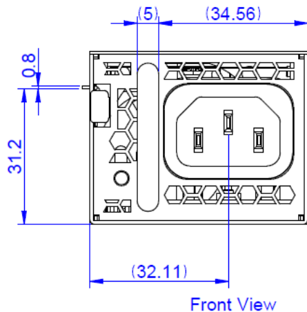
Figure 15 – Front View
