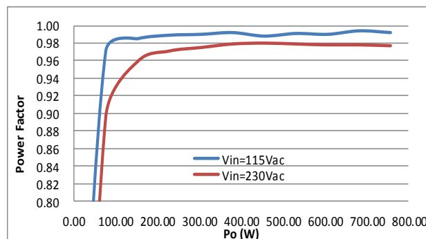
Figure 3 - Power factor vs. Load current
