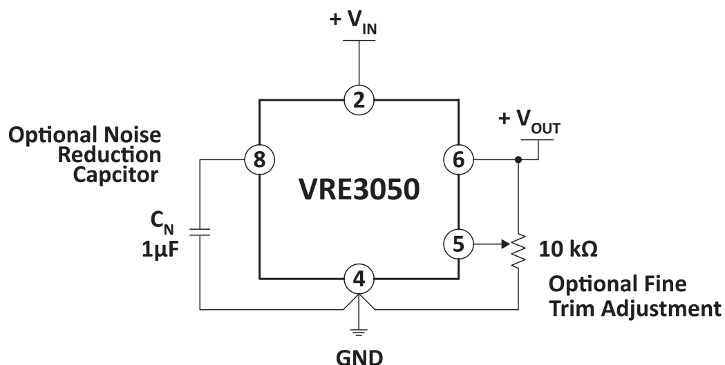
Figure 1: Typical Connection
