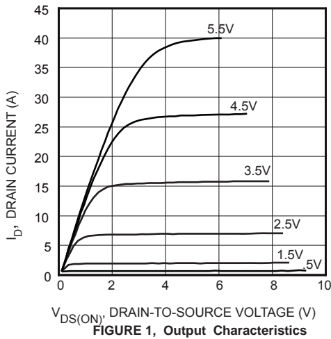
FIGURE 1, Output Characteristics
