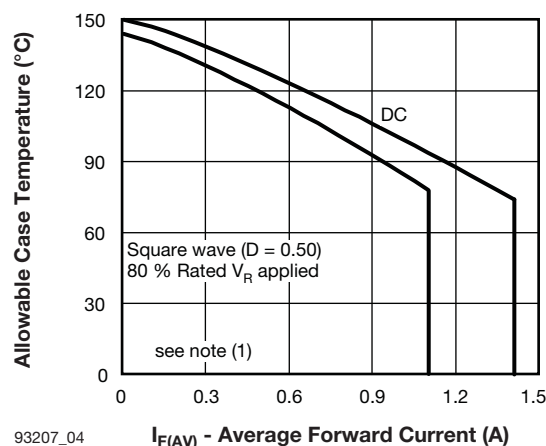
Fig. 4 - Maximum Ambient Temperature vs. Average Forward Current
