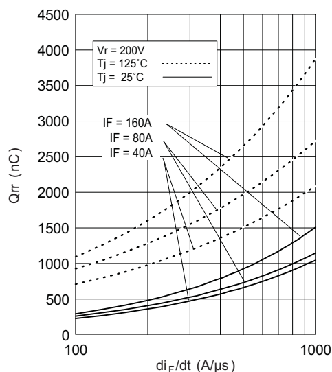
Fig. 6 - Typical Stored Charge vs. dI_F/dt
