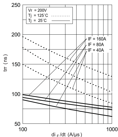
Fig. 5 - Typical Reverse Recovery Time vs. dI_F/dt
