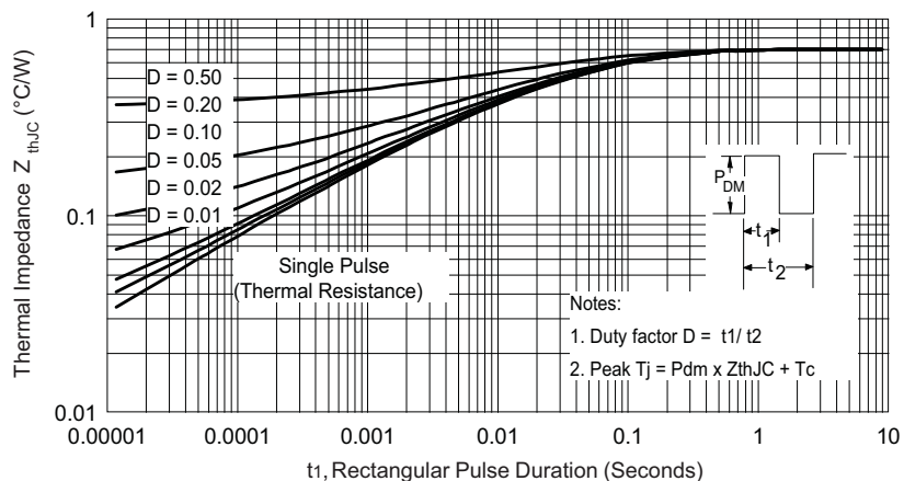
Fig. 3 - Maximum Thermal Impedance Z_{thJC} Characteristics
