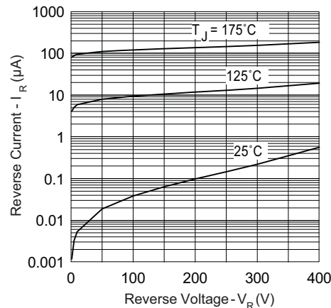
Fig. 1 - Typical Values of Reverse Current vs. Reverse Voltage
