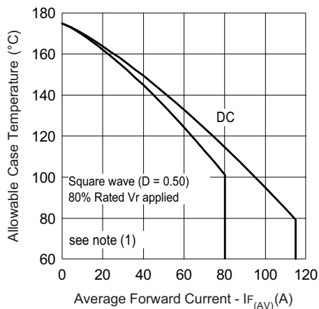
Fig. 2 - Maximum Allowable Case Temperature vs. Average Forward Current
