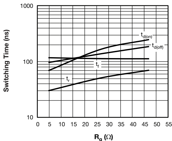
Fig. 29 - Typical Q2 - Q3 Trench IGBT 600 V Switching Time vs. R_g (with Freewheeling External TO-247 Diode Discrete 30ETH06) T_J = 125^\circ\text{C} , V_{CC} = 300\text{ V} , I_C = 30\text{ A} , V_{GE} = 15\text{ V} , L = 500\text{ }\mu\text{H}
