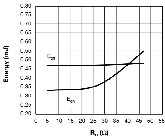
Fig. 28 - Typical Q2 - Q3 Trench IGBT 600 V Energy Loss vs. R_g (with Freewheeling External TO-247 Diode Discrete 30ETH06) T_J = 125^\circ\text{C} , V_{CC} = 300\text{ V} , I_C = 30\text{ A} , V_{GE} = 15\text{ V} , L = 500\text{ }\mu\text{H}
