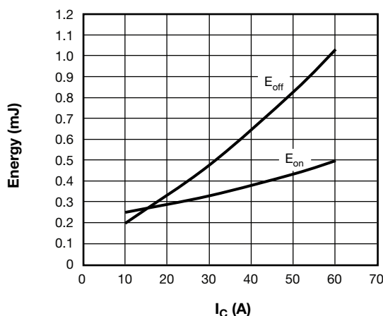
Fig. 26 - Typical Q2 - Q3 Trench IGBT 600 V Energy Loss vs. I_C (with Freewheeling External TO-247 Diode Discrete 30ETH06 ) T_J = 125\text{ °C} , V_{CC} = 300\text{ V} , R_g = 4.7\text{ }\Omega , V_{GE} = 15\text{ V} , L = 500\text{ }\mu\text{H}
