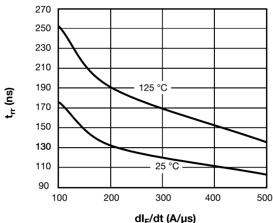
Fig. 13 - Typical D1 - D4 Antiparallel Diode Reverse Recovery Time vs. dI_F/dt V_{rr} = 400 V, I_F = 20 A
