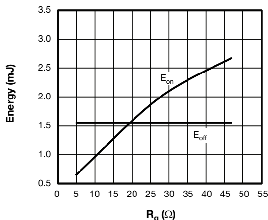
Fig. 9 - Typical Q1 - Q4 Trench IGBT 1200 V Energy Loss vs. R_g (with D1 - D4 Freewheeling Diode) T_J = 125^\circ\text{C} , V_{CC} = 600\text{ V} , I_C = 30\text{ A} , V_{GE} = 15\text{ V} , L = 500\ \mu\text{H}
