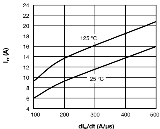
Fig. 14 - Typical D1 - D4 Antiparallel Diode Reverse Recovery Current vs. dI_F/dt V_{rr} = 400 V, I_F = 20 A
