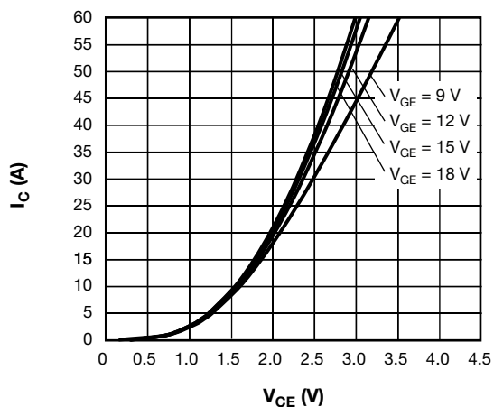
Fig. 2 - Typical Q1 - Q4 Trench IGBT 1200 V Output Characteristics T_J = 125^\circ\text{C}
