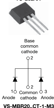
TO-262AA
