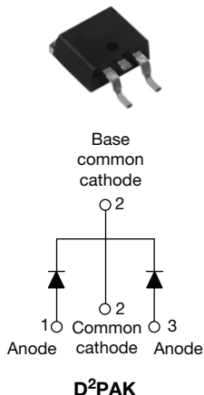
VS-MBRB15..CTPbF
