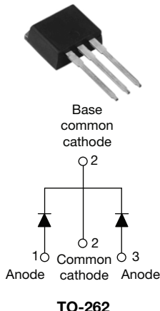
VS-MBR15..CT-1PbF
