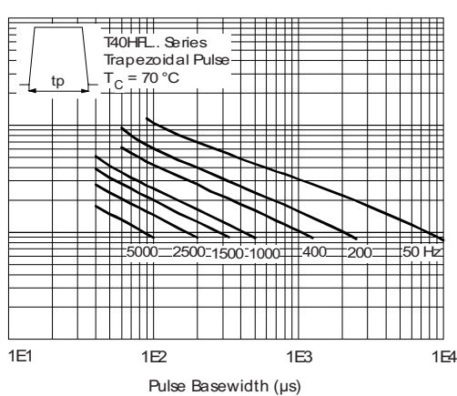
Fig. 37 - Frequency Characteristics
