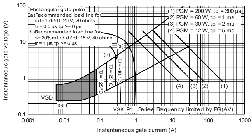
Fig. 12 - Gate Characteristics
