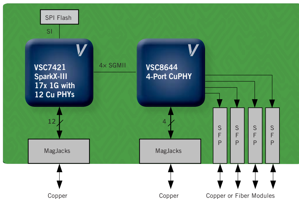
VSC7421 in a 16-port 1-GbE switch application
