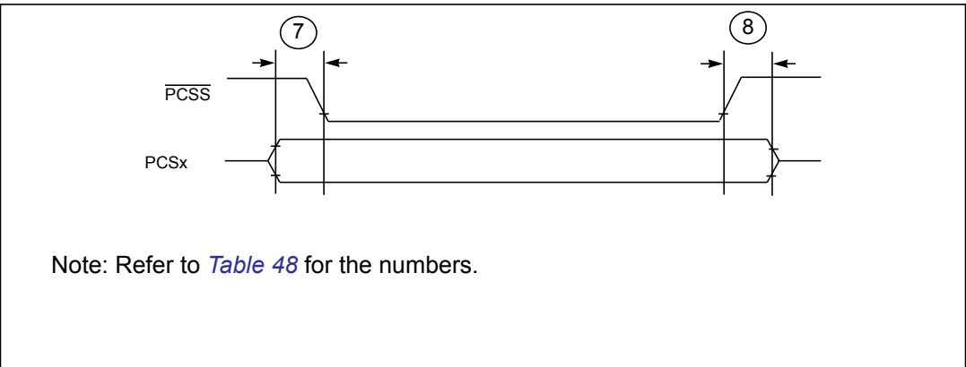
Figure 31. DSPI PCS strobe ( \overline{\text{PCSS}} ) timing
