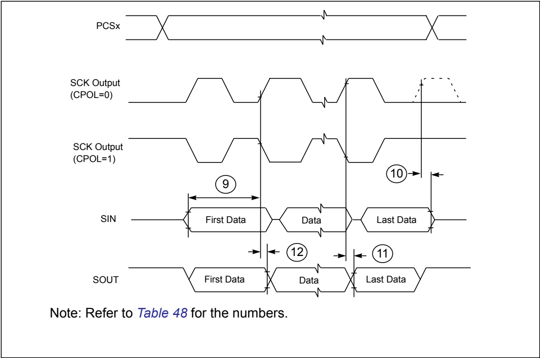
Figure 28. DSPI modified transfer format timing — master, CPHA = 1
