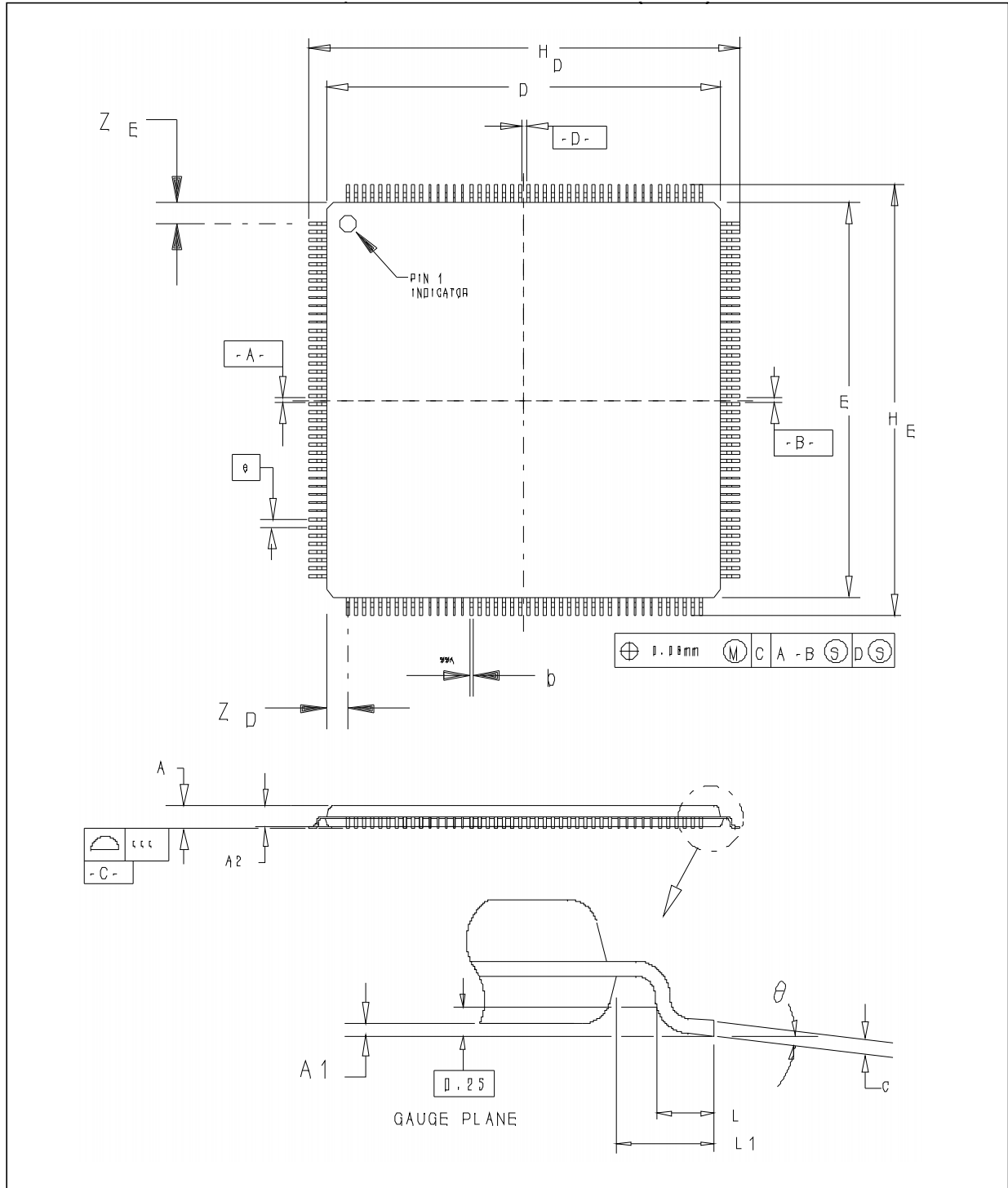
Figure 33. LQFP176 package mechanical drawing
