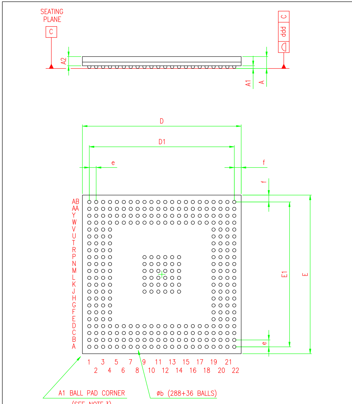
Figure 34. PBGA324 package mechanical drawing
