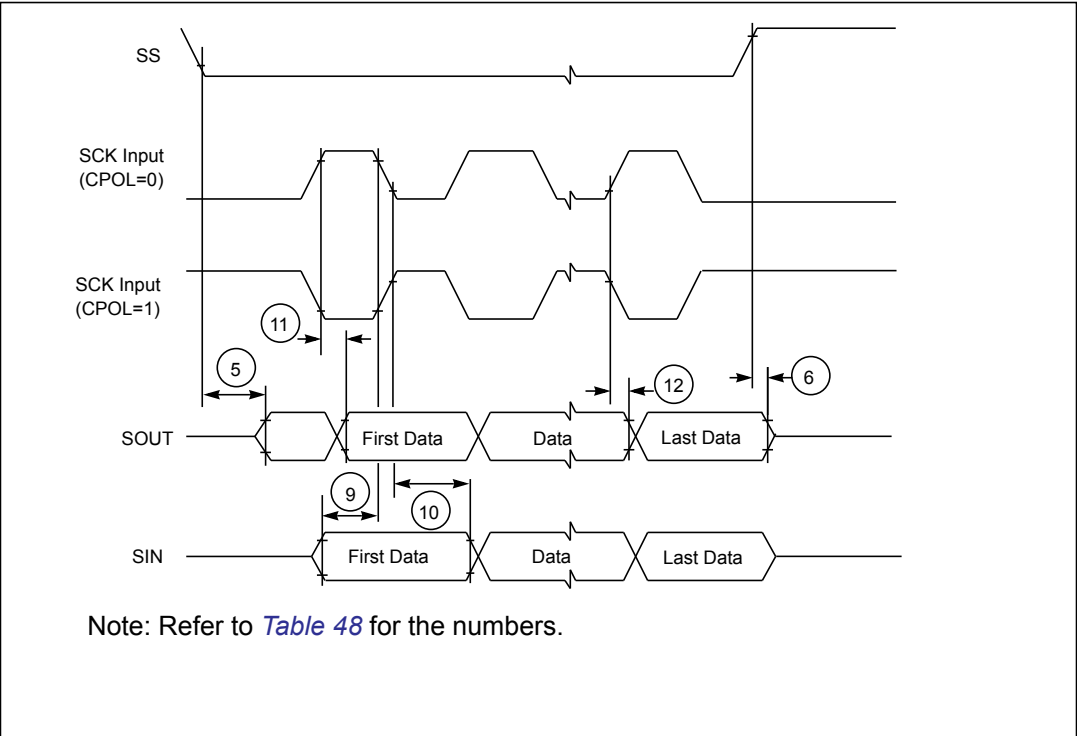
Figure 30. DSPI modified transfer format timing — slave, CPHA =1
