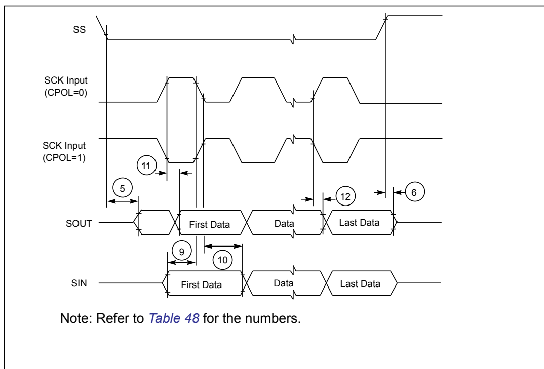
Figure 26. DSPI classic SPI timing — slave, CPHA = 1
