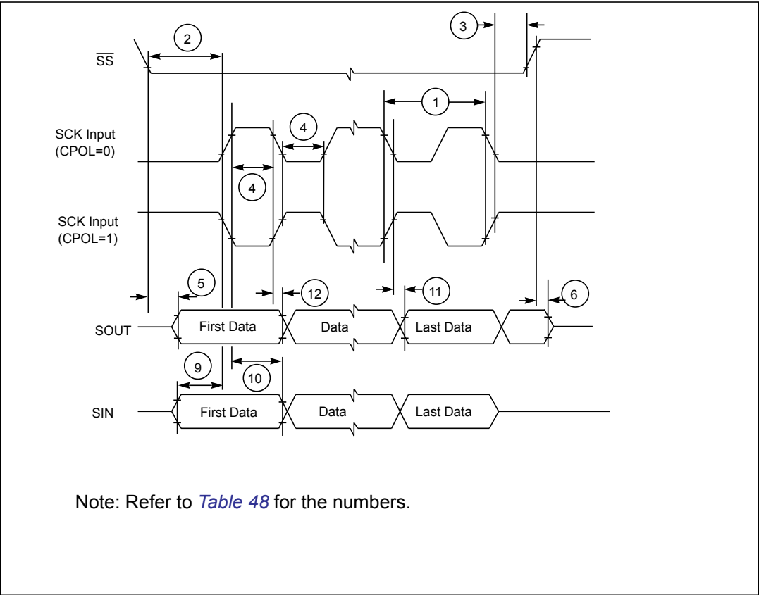
Figure 25. DSPI classic SPI timing — slave, CPHA = 0
