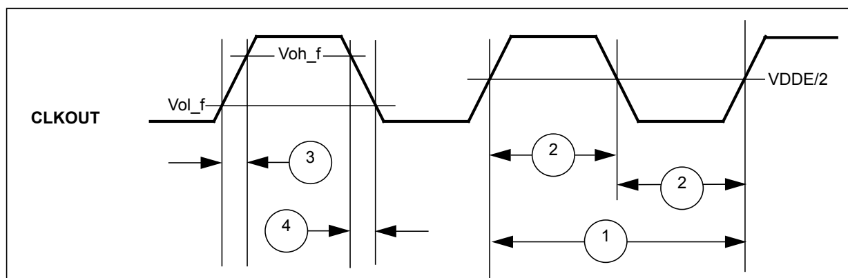
Figure 18. CLKOUT timing
