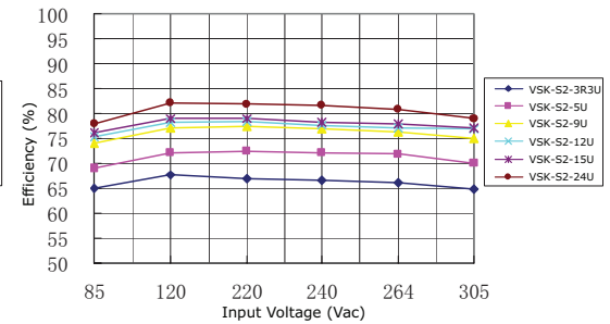
3. efficiency vs. input voltage (load=100%)
