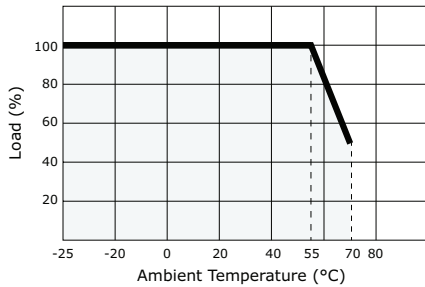
1. output power vs. ambient temperature (85~305 Vac)
