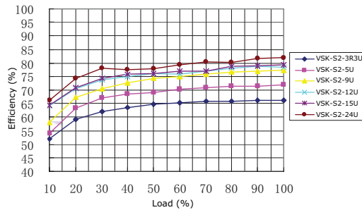
2. efficiency vs. output power (Vin=220Vac)
