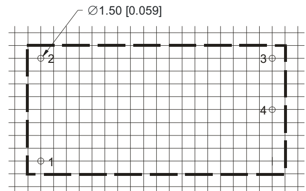
Top View PCB LAYOUT
