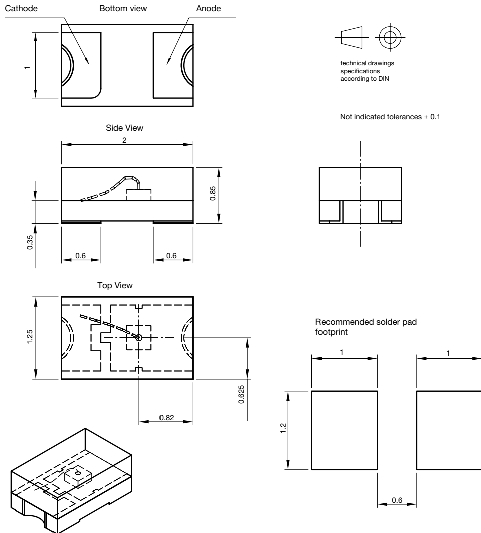
Drawing-No.: 6.541-5083.01-4 Issue: 2; 10.09.2013
