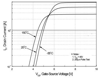
Figure 2. Transfer Characteristics
