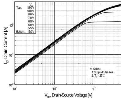
Figure 1. On-Region Characteristics
