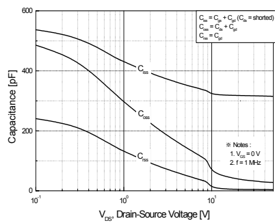
Figure 5. Capacitance Characteristics
