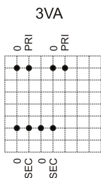
5.08mm Grid Pin View
