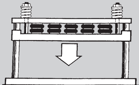
GLUING PRESS
