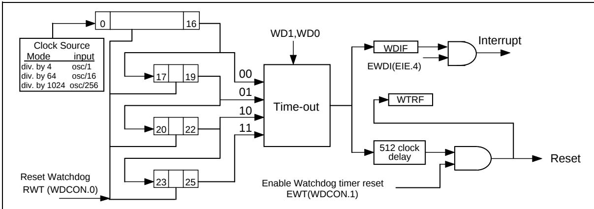
Figure 19. Watchdog Timer
