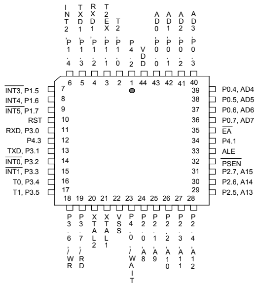
44-Pin PLCC
