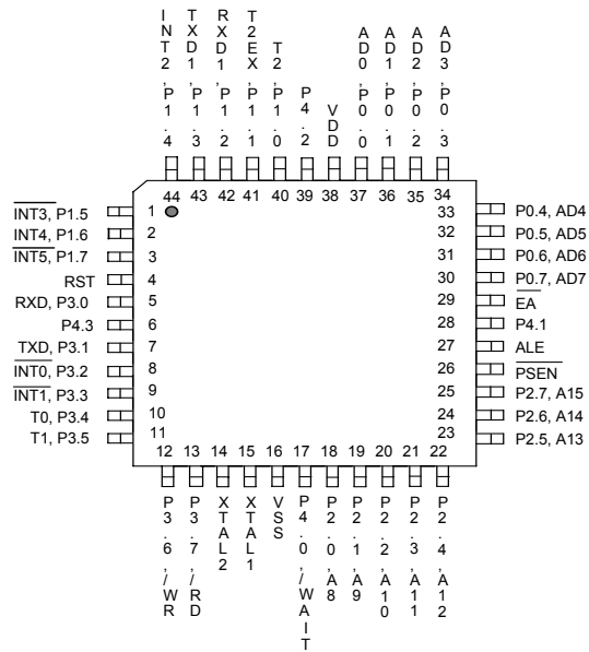
44-Pin QFP
