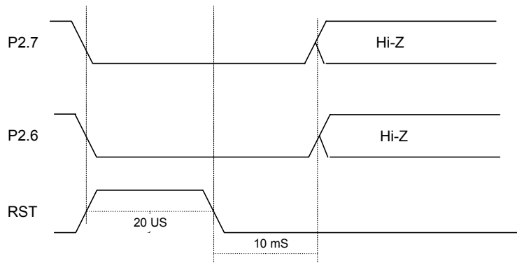
The Reset Timing For Entering REBOOT Mode
