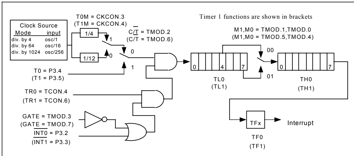
Figure 11. Timer/Counter Mode 0 &amp; Mode 1
