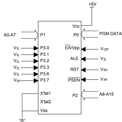
Programming Configuration
