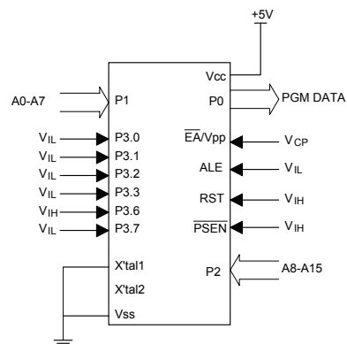
Programming Verification
