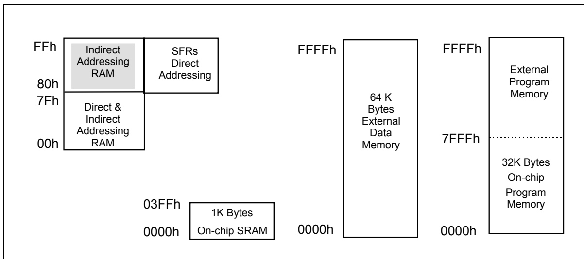
Figure 1. Memory Map
