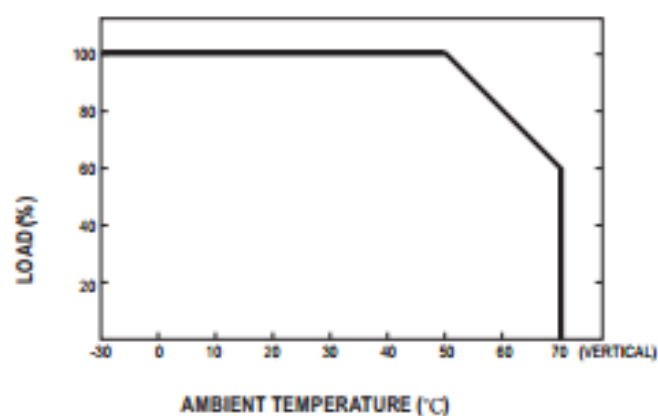
■ Derating Curve
