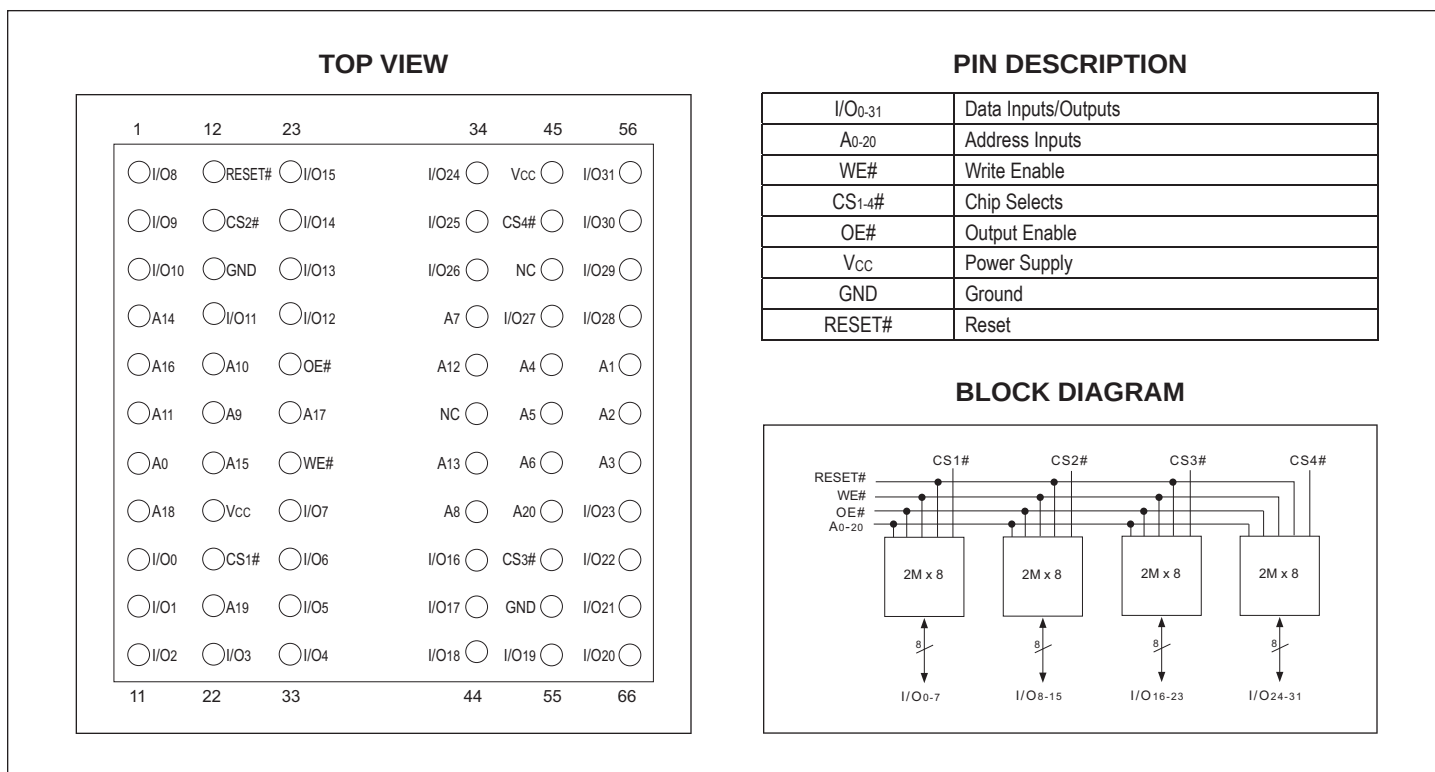
FIGURE 10 – ALTERNATE PIN CONFIGURATION FOR WF2M32I-XHX5
