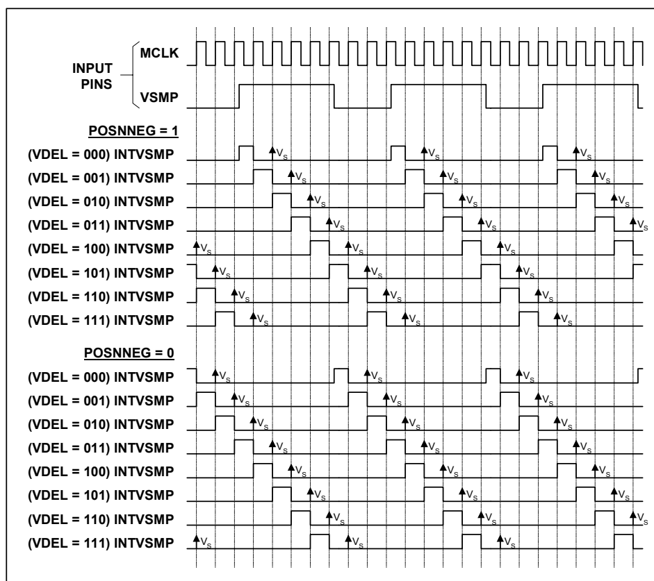
Figure 20 Internal VSMP Pulses Generated by Programmable VSMP Detect Circuit
