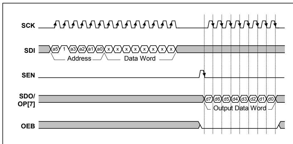
Figure 19 Serial Interface Register Read-back
