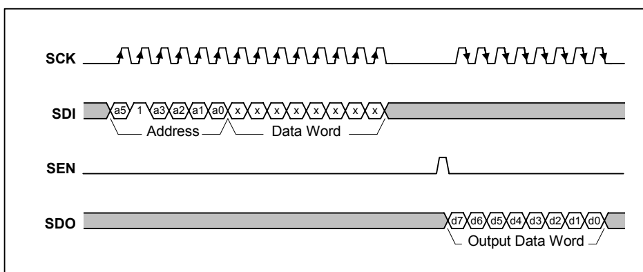
Figure 16 Serial Interface Register Read-back
