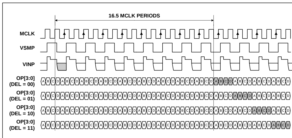
Figure 16 Mode 3 Operation
