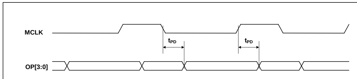
Figure 2 Output Data Timing
