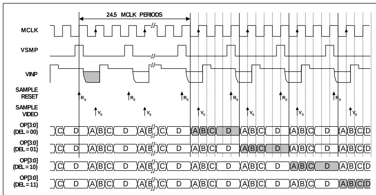
Figure 15 Mode 2 Operation
