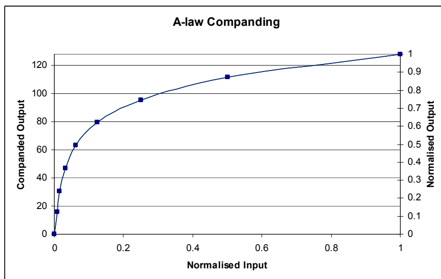
Figure 54 A-Law Companding
