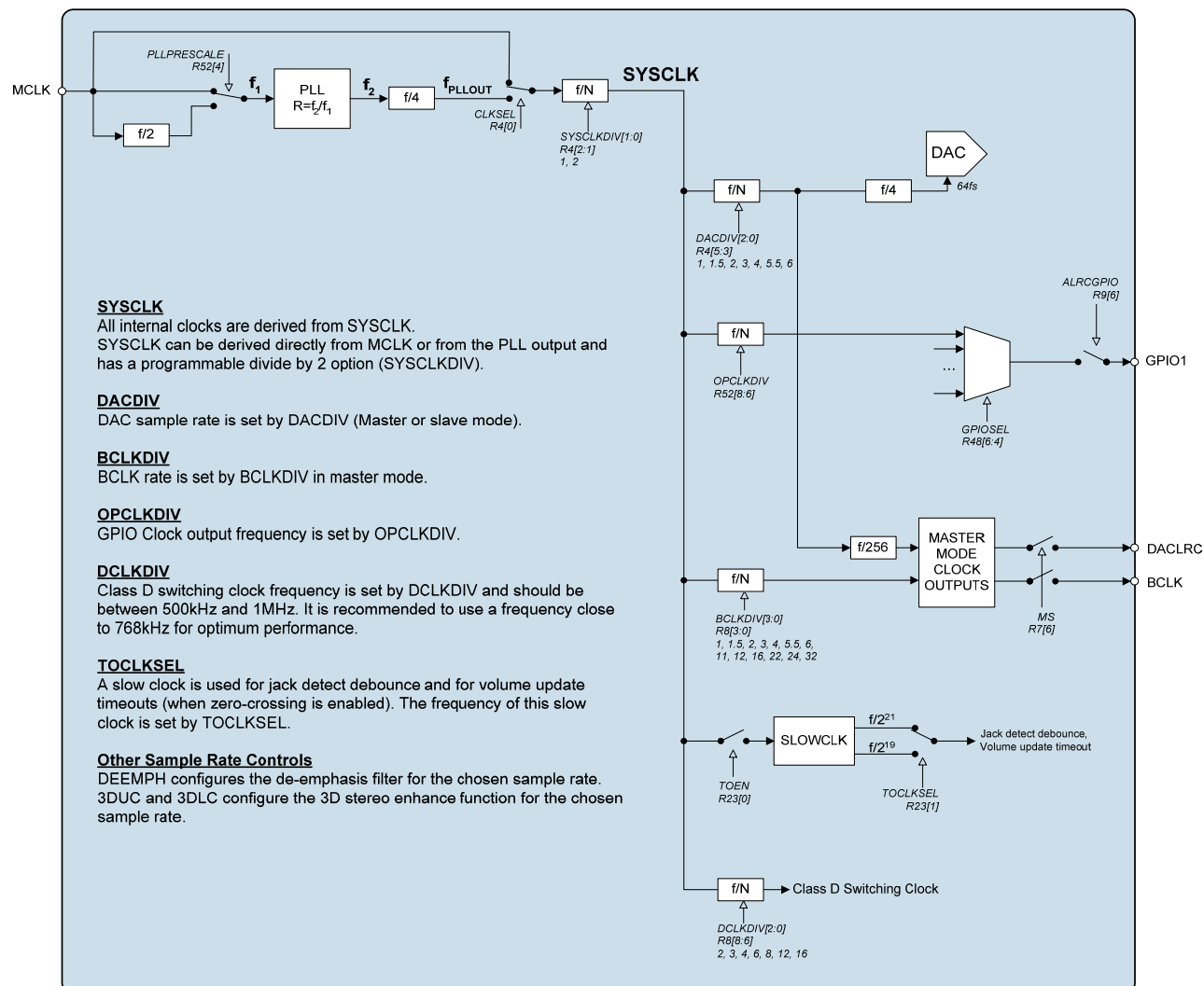
Figure 34 Clocking Scheme
