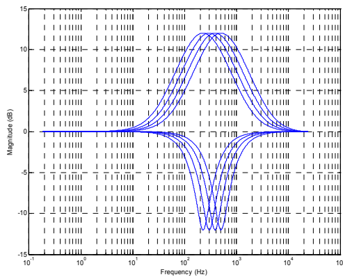
Figure 66 EQ Band 2 – Peak Filter Centre Frequencies, EQ2BW=0
