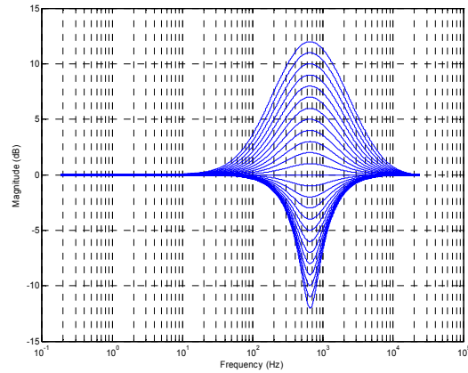
Figure 70 EQ Band 3 – Peak Filter Gains for Lowest Cut-off Frequency, EQ3BW=0
