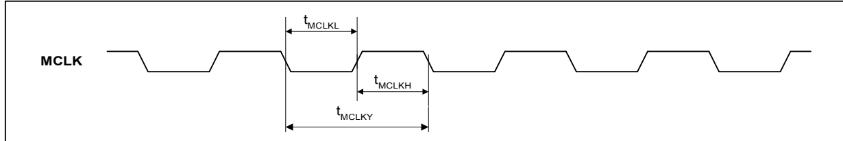
Figure 5 System Clock Timing Requirements
