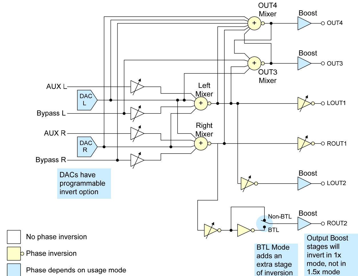
Figure 40 Output Signal Path Phasing
