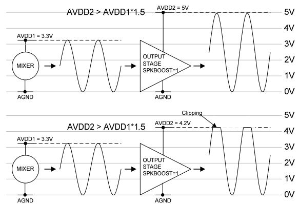
Figure 36 Boost Mode Output Operation
