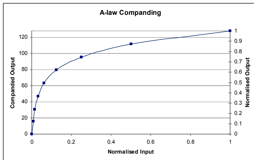
Figure 51 A-Law Companding
