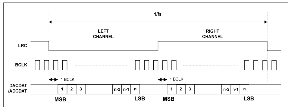
Figure 44 I^2S Audio Interface (assuming n-bit word length)
