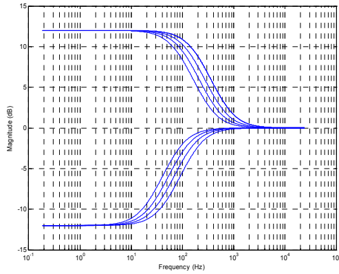
Figure 64 EQ Band 1 Low Frequency Shelf Filter Cut-offs
