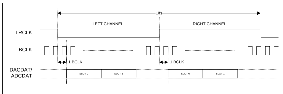
Figure 59 TDM in I 2 S Mode
