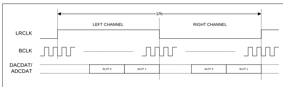
Figure 57 TDM in Right-Justified Mode
