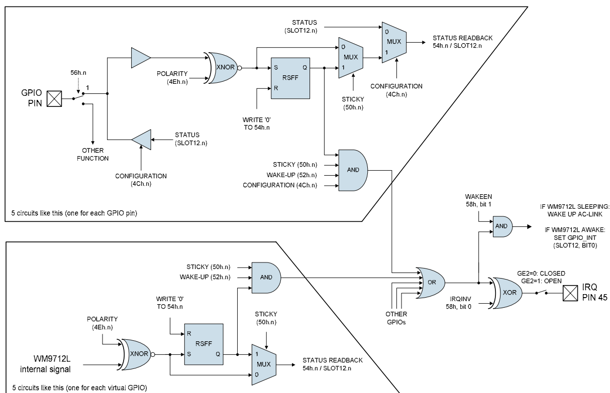
Figure 15 GPIO logic
