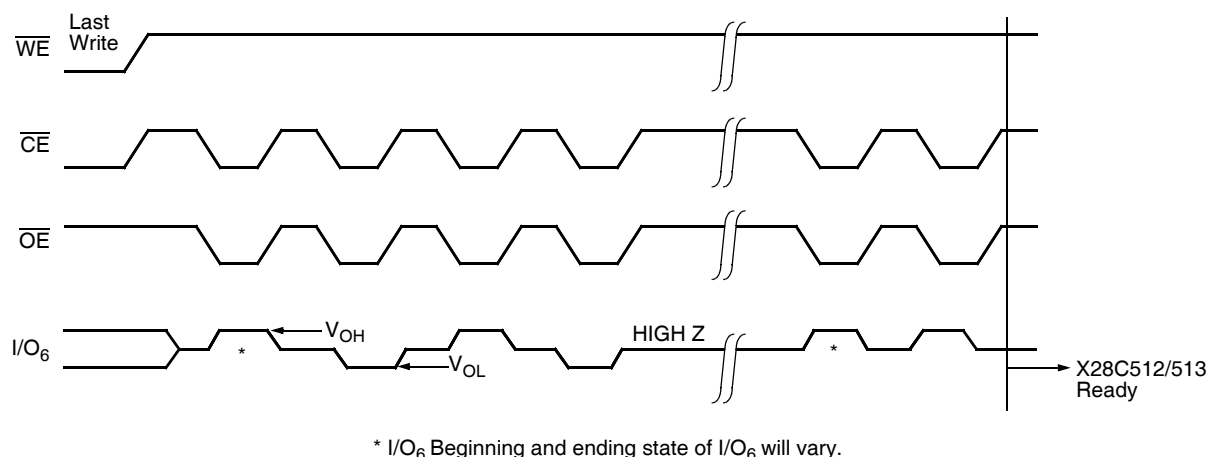
Figure 4. Toggle Bit Bus Sequence
